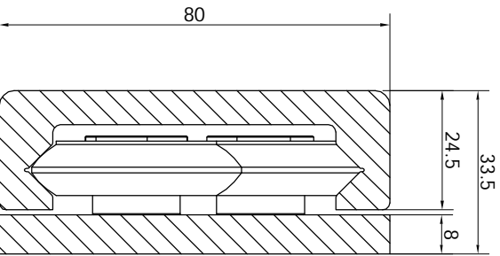
SECTION (Scale 2:1)
